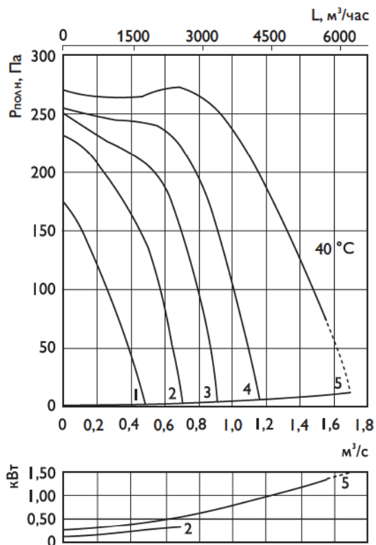
RK 800×500 C3/RKC 500 C3
